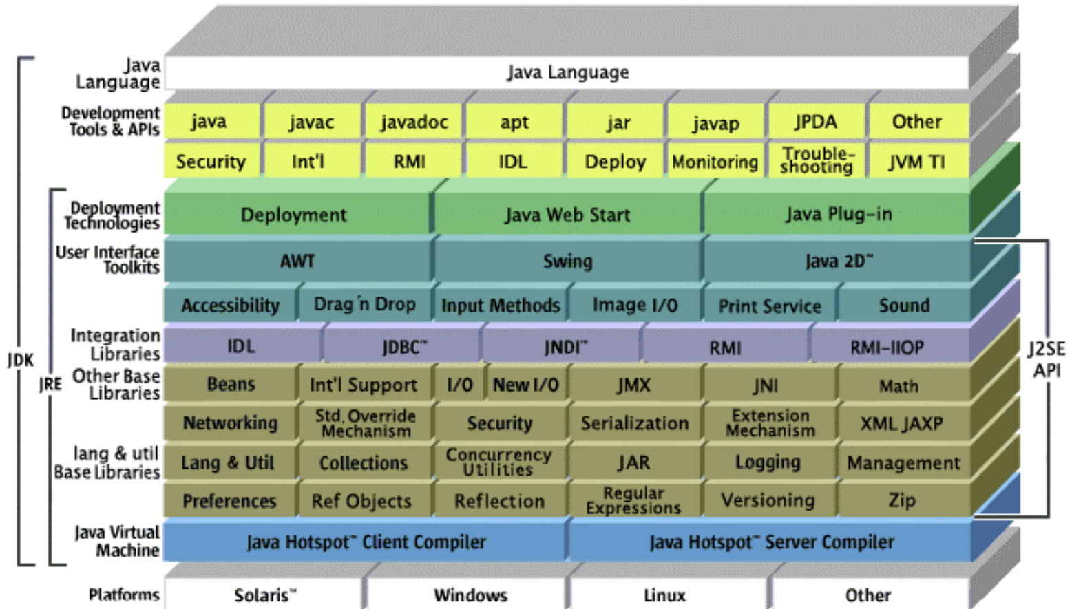
Java™ 2 Platform Standard Edition 5.0
